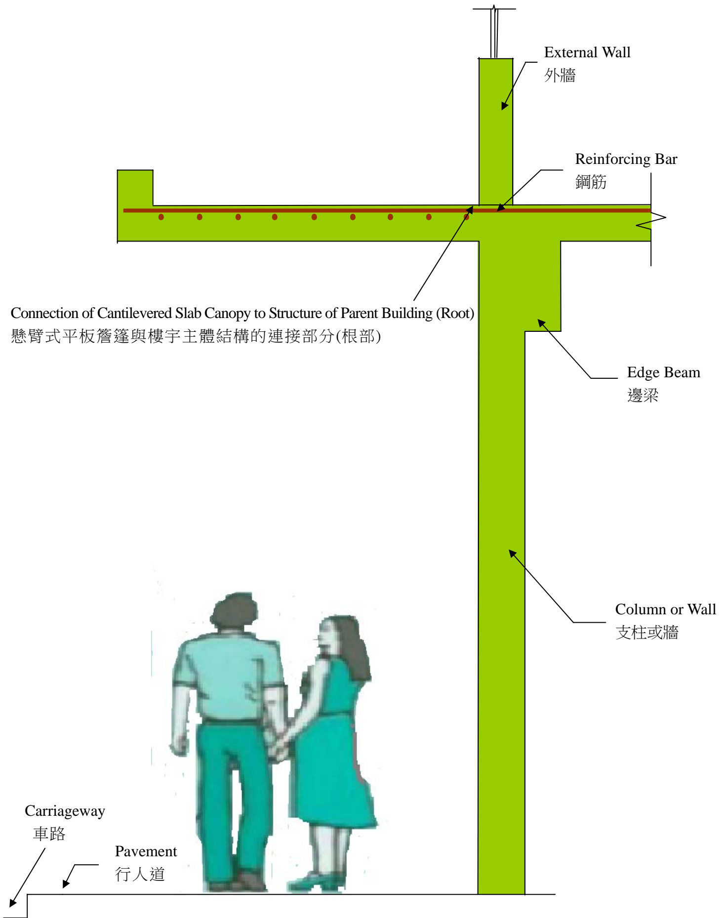
Typical Cantilevered Slab Canopy
