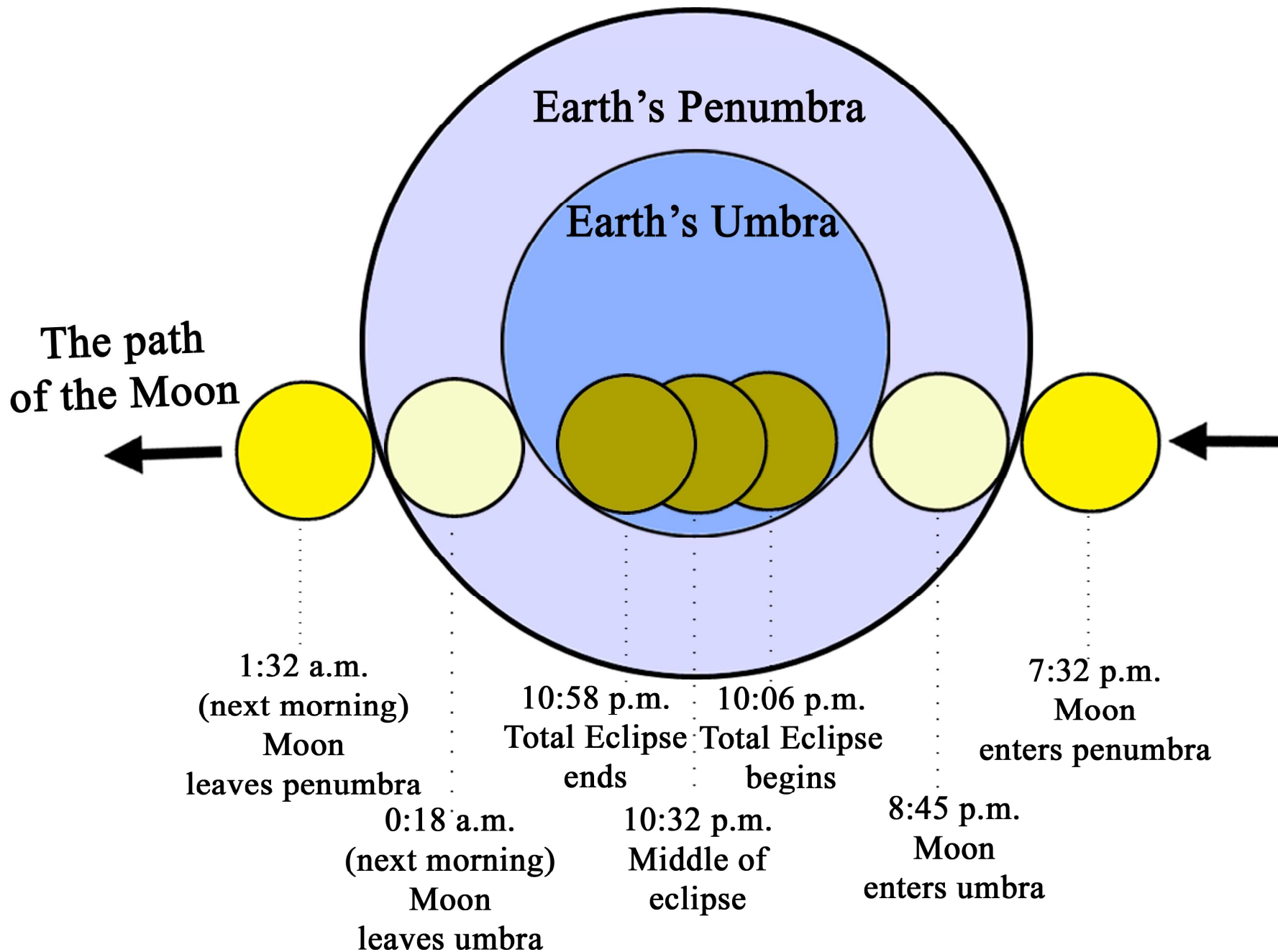
The path of the moon during the eclipse on December 10, 2011
