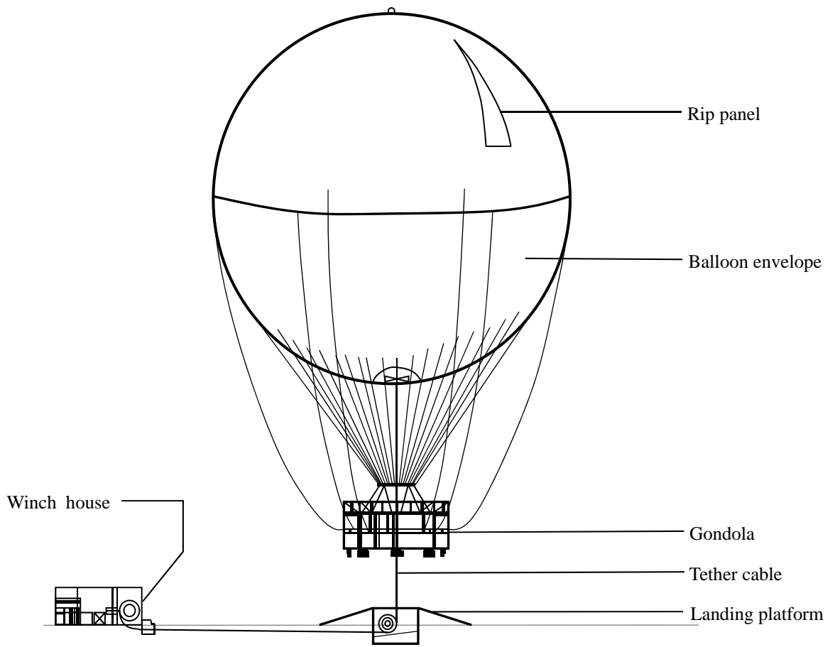
Schematic diagram of Helium Balloon Ride
