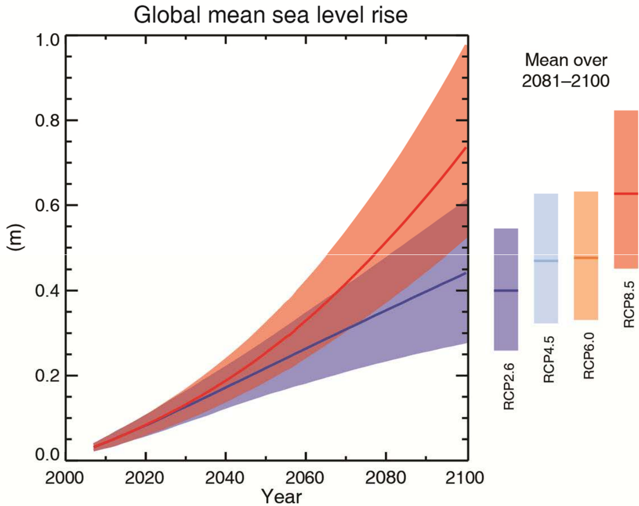
Figure 2: Projections of global mean sea level rise over the 21st century relative to 1986-2005
