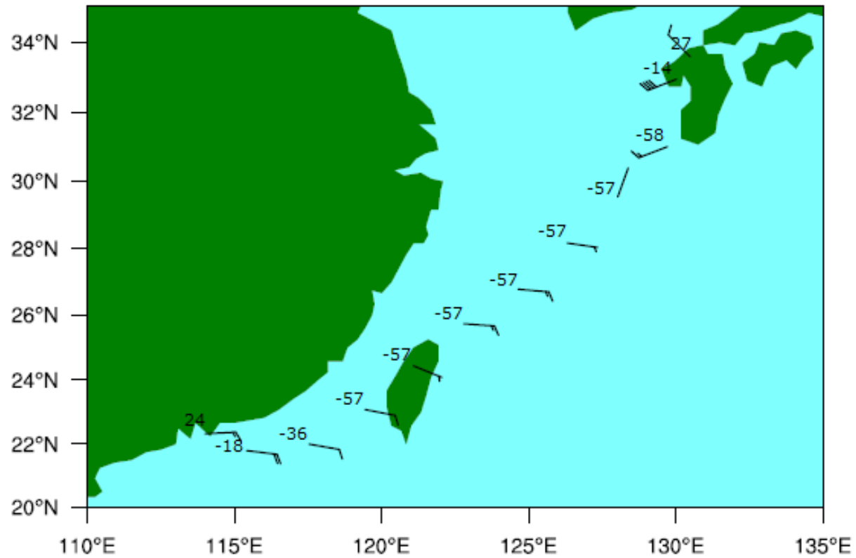
Figure 1: First weather observations received from an aircraft of Hong Kong Dragon Airlines Limited (July 17, 2014)
