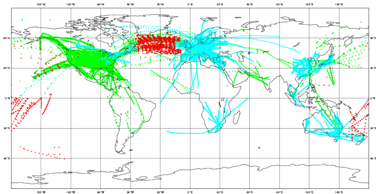
Figure 2: Global Aircraft Meteorological Data Relay observations between 2pm and 8pm on August 6, 2014
