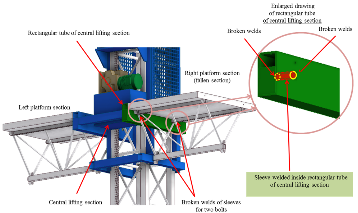
Figure 2: Connection between right platform and central lifting section
