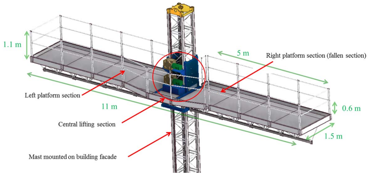
Figure 1: Illustration of tower working platform
