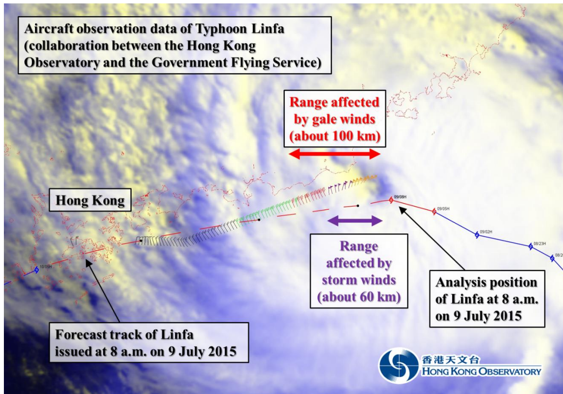
Aircraft observation data collected near Typhoon Linfa (collaboration between the Observatory and the Government Flying Service).
