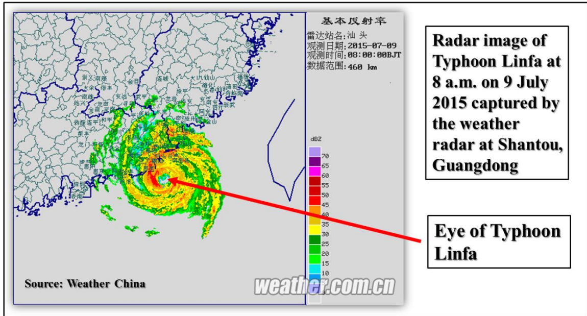
Weather radar image at Shantou, 8 a.m. on 9 July 2015.
