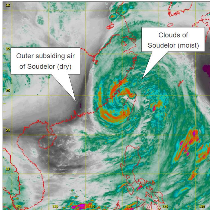
Figure 2: Water vapour satellite image of 1 pm, August 8, 2015 which shows the moist and dry regions. The satellite image is generated with satellite data from the Japan Meteorological Agency.
