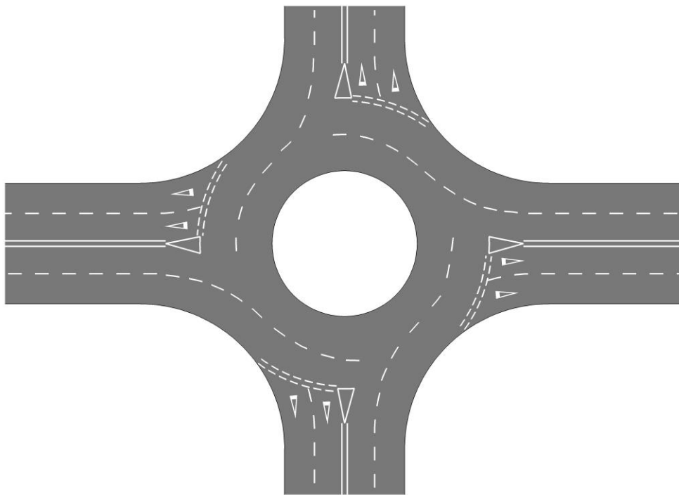
Figure 2 : Spiral Roundabout
