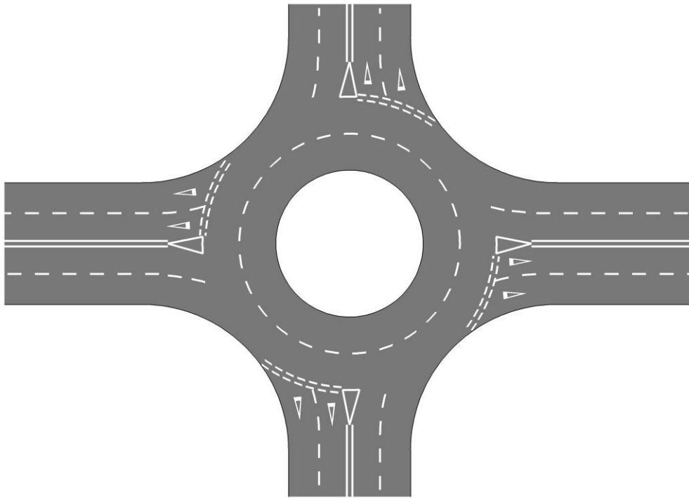
Figure 2 : Spiral Roundabout
