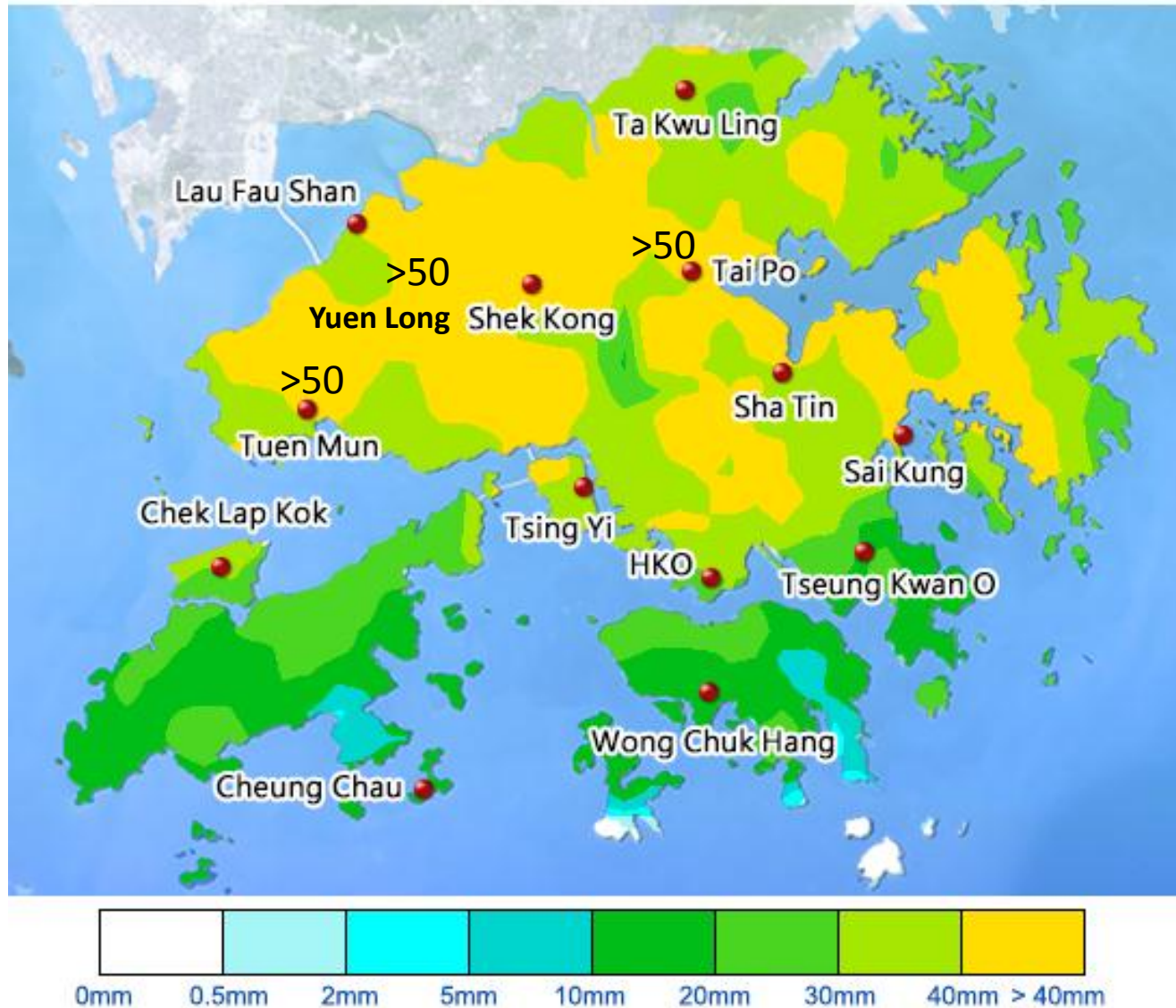
Figure 2 Rainfall distribution map for the hour ending 7.45a.m. (> 50 represents regions with rainfall exceeding 50 mm in an hour)
