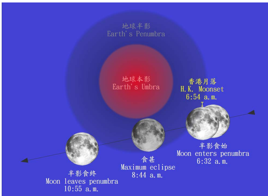
Path of the moon during the penumbral lunar eclipse on February 11
