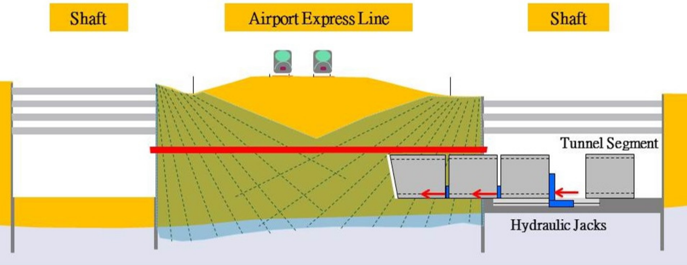
Box-jacking of tunnel segments in Scenic Hill Tunnel by hydraulic jacks underneath Airport Express Line
