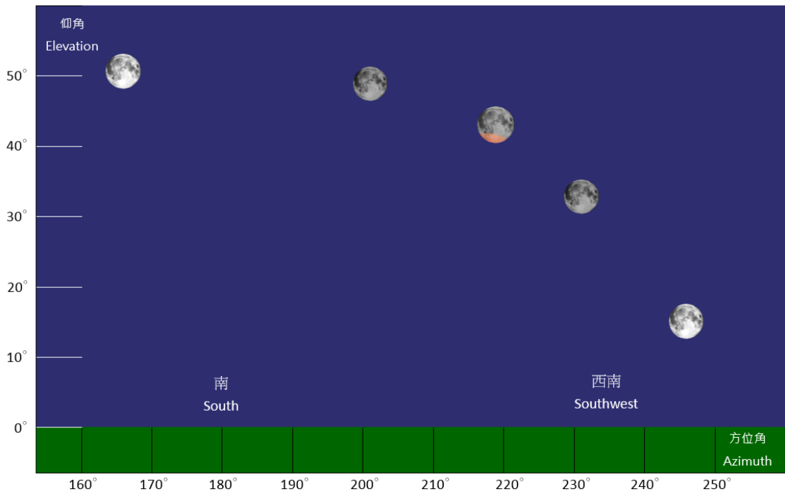
Figure 2 Schematic diagram showing positions (elevation and azimuth) of the moon during the partial lunar eclipse on August 7 to 8, 2017
