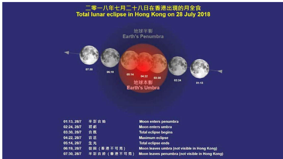
Figure 2 The total lunar eclipse process on July 28
