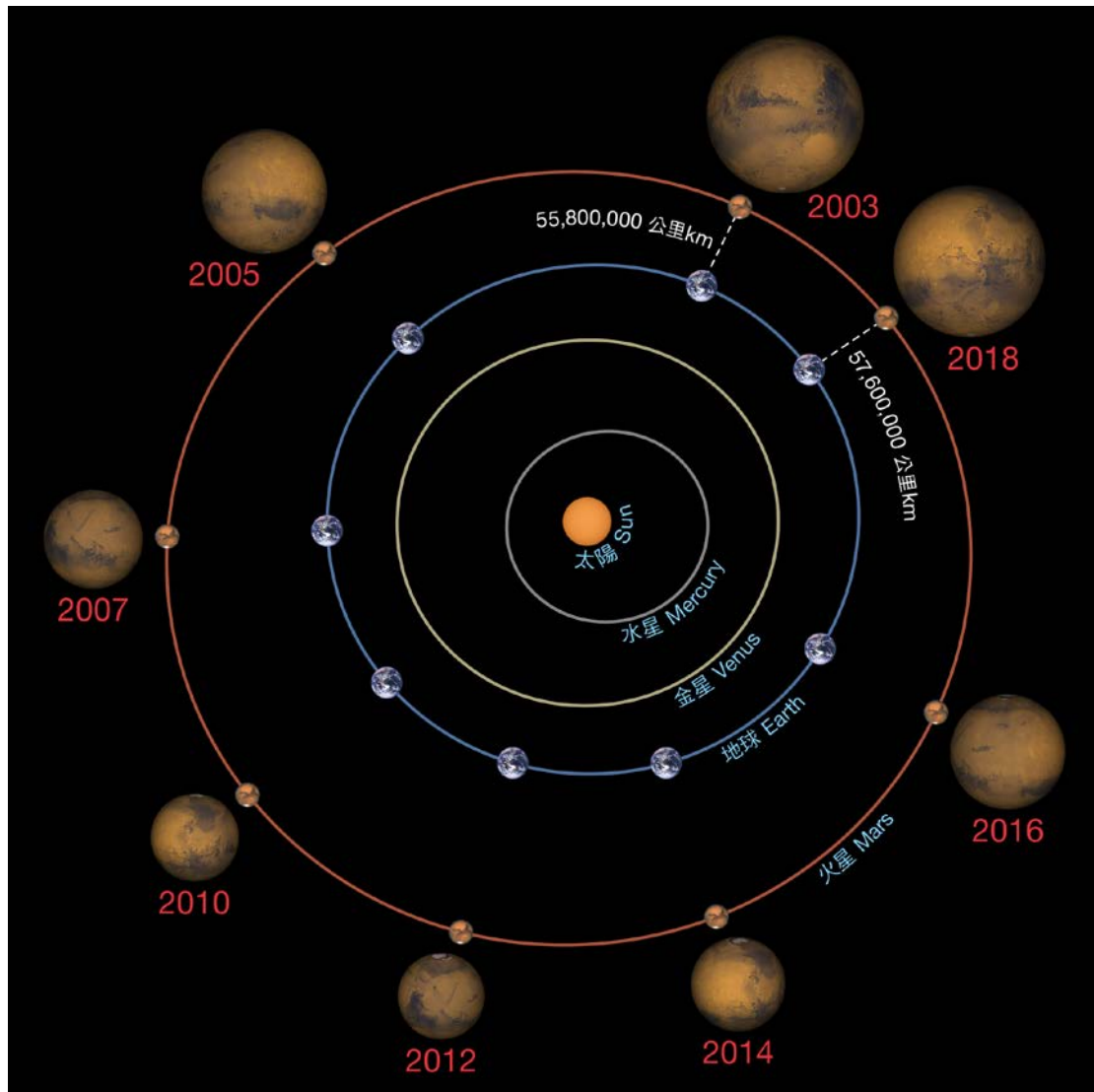
Figure 1 Mars Opposition from 2003 to 2018 (Courtesy of Hong Kong Space Museum)
