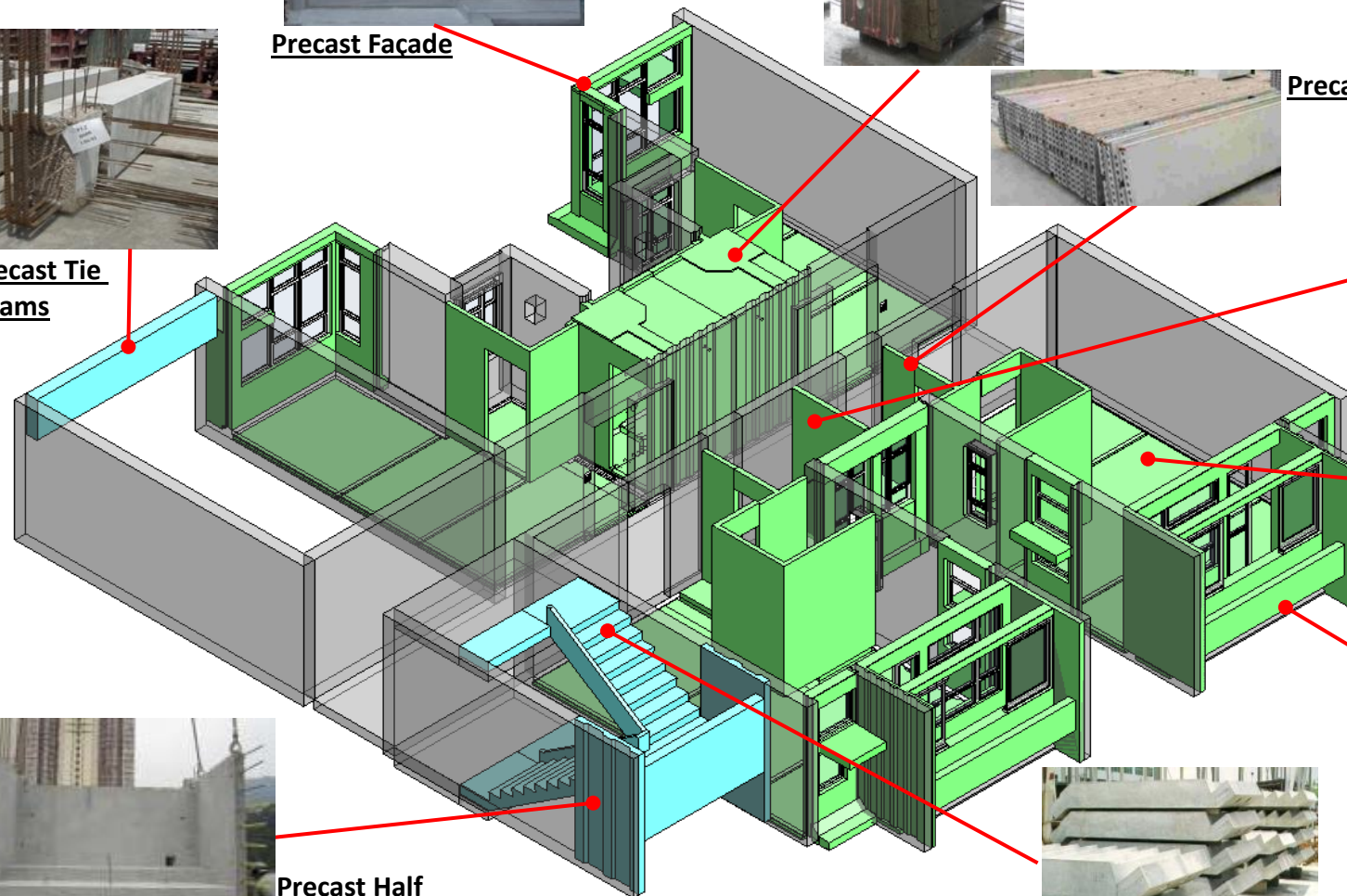
Precast Staircase
