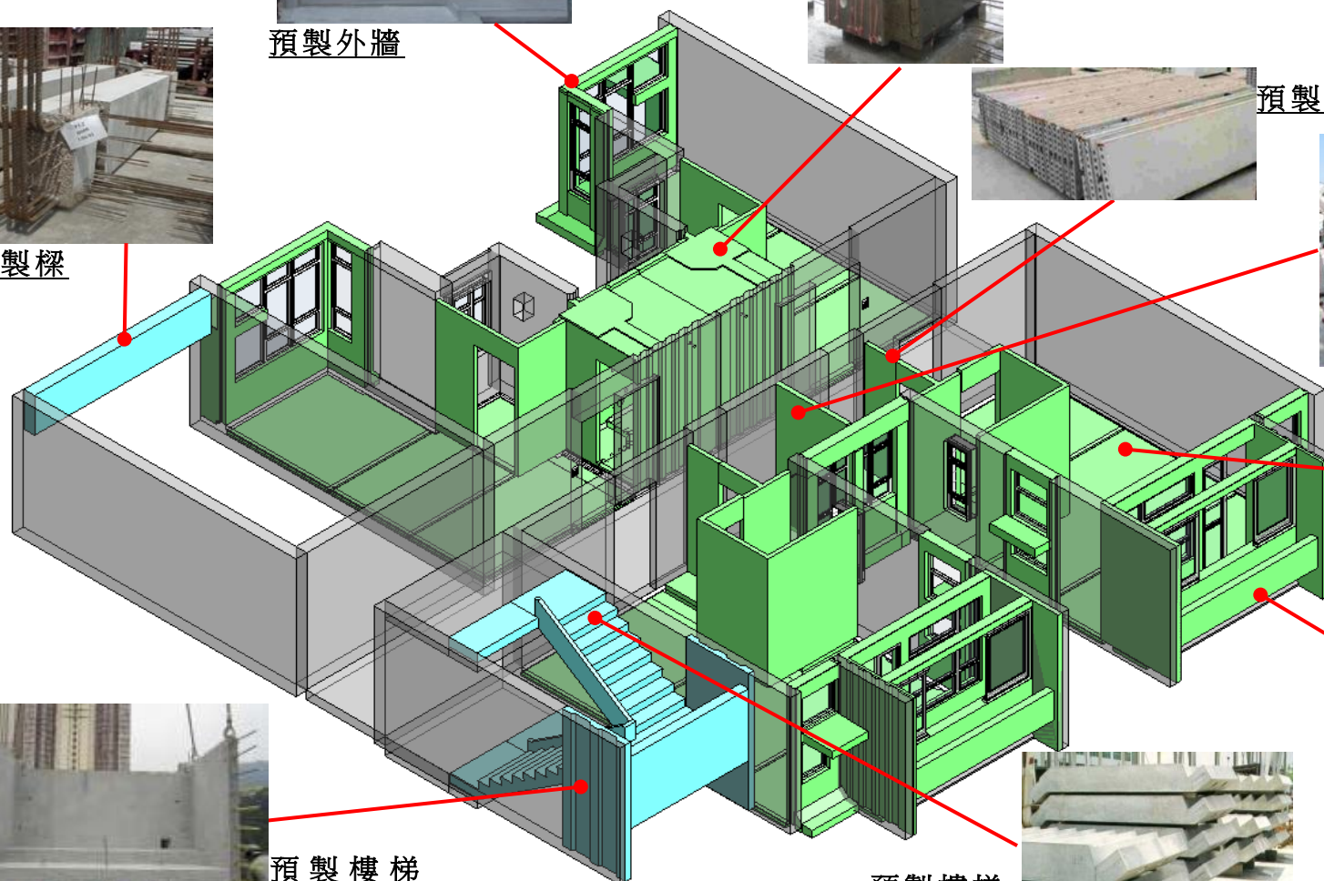
預製樓梯
