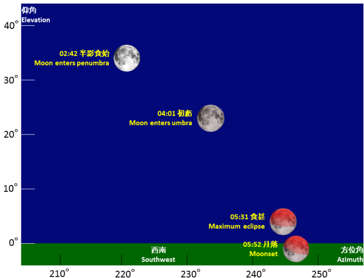
Figure 2 Schematic diagram showing elevation and azimuth of the moon during the partial lunar eclipse on July 17, 2019
