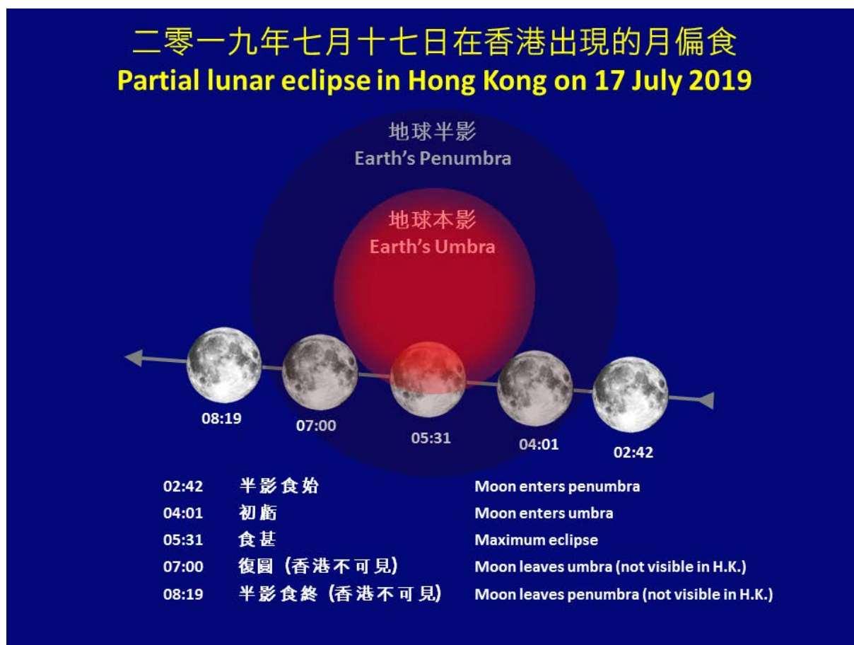
Figure 1 The partial lunar eclipse process on July 17, 2019
