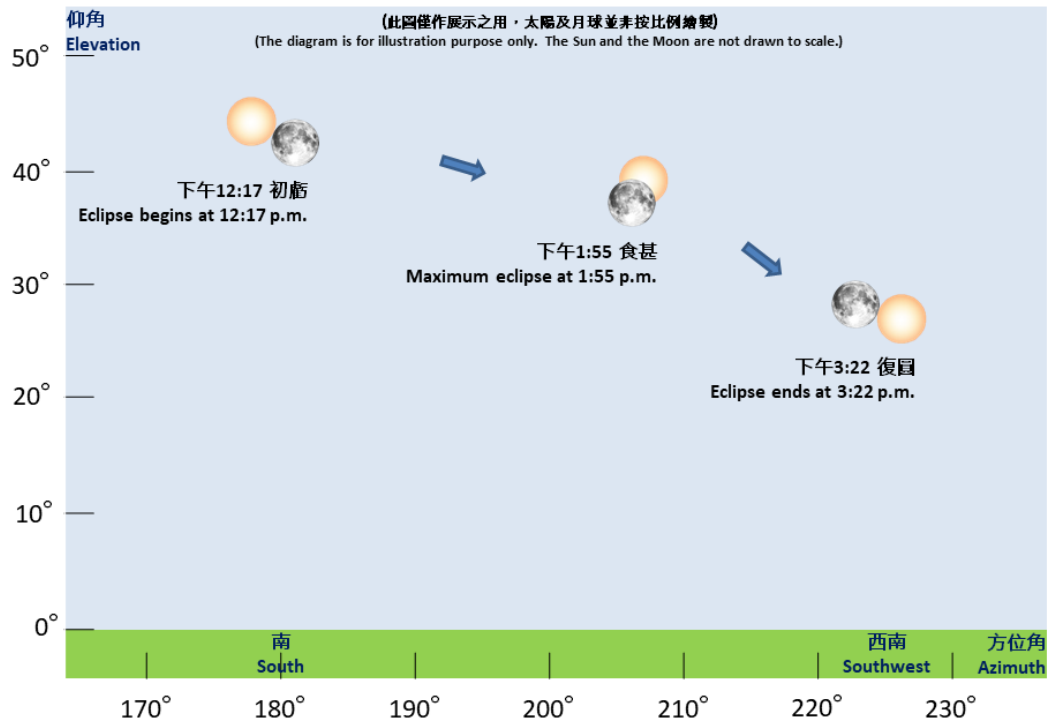
Schematic diagram showing elevation and azimuth of the Sun and the Moon during the partial solar eclipse on December 26, 2019
