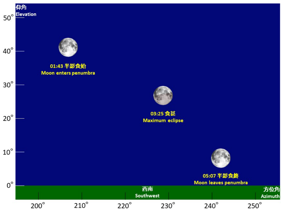
Figure 2 Schematic diagram showing elevation and azimuth of the moon during the penumbral eclipse on June 6, 2020
