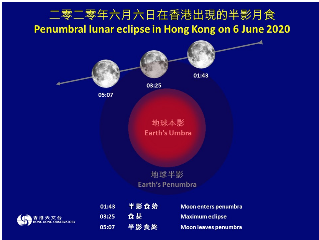
Figure 1 The penumbral lunar eclipse process on June 6, 2020
