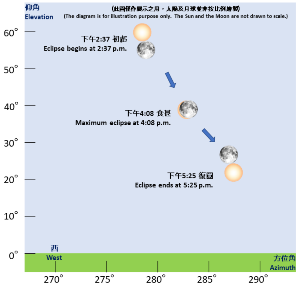
Schematic diagram showing elevation and azimuth of the sun and the moon during the partial solar eclipse on June 21, 2020
