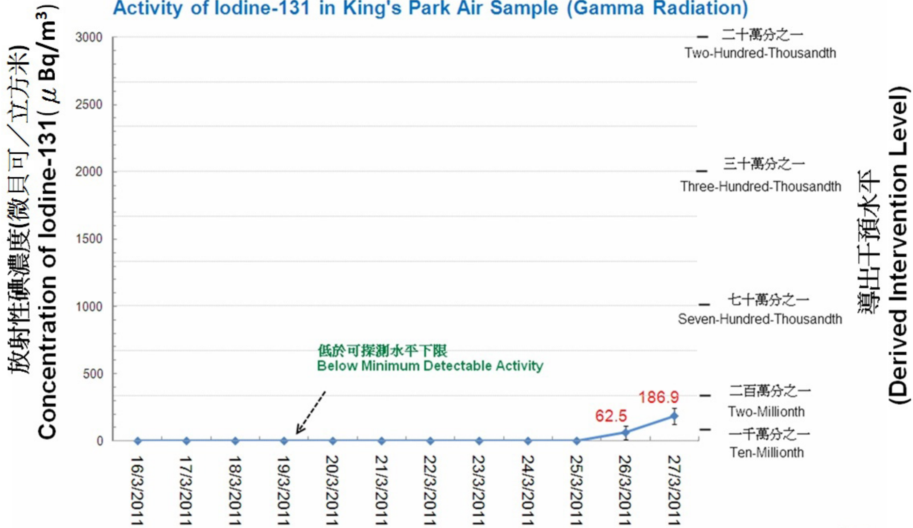
Figure 1 The activity of Iodine-131 in air samples measured at King's Park. Please note that the date in the figure is the starting date for air sampling. For example, 26 March corresponds to the air sample taken between noon, 26 March and noon, 27 March.
