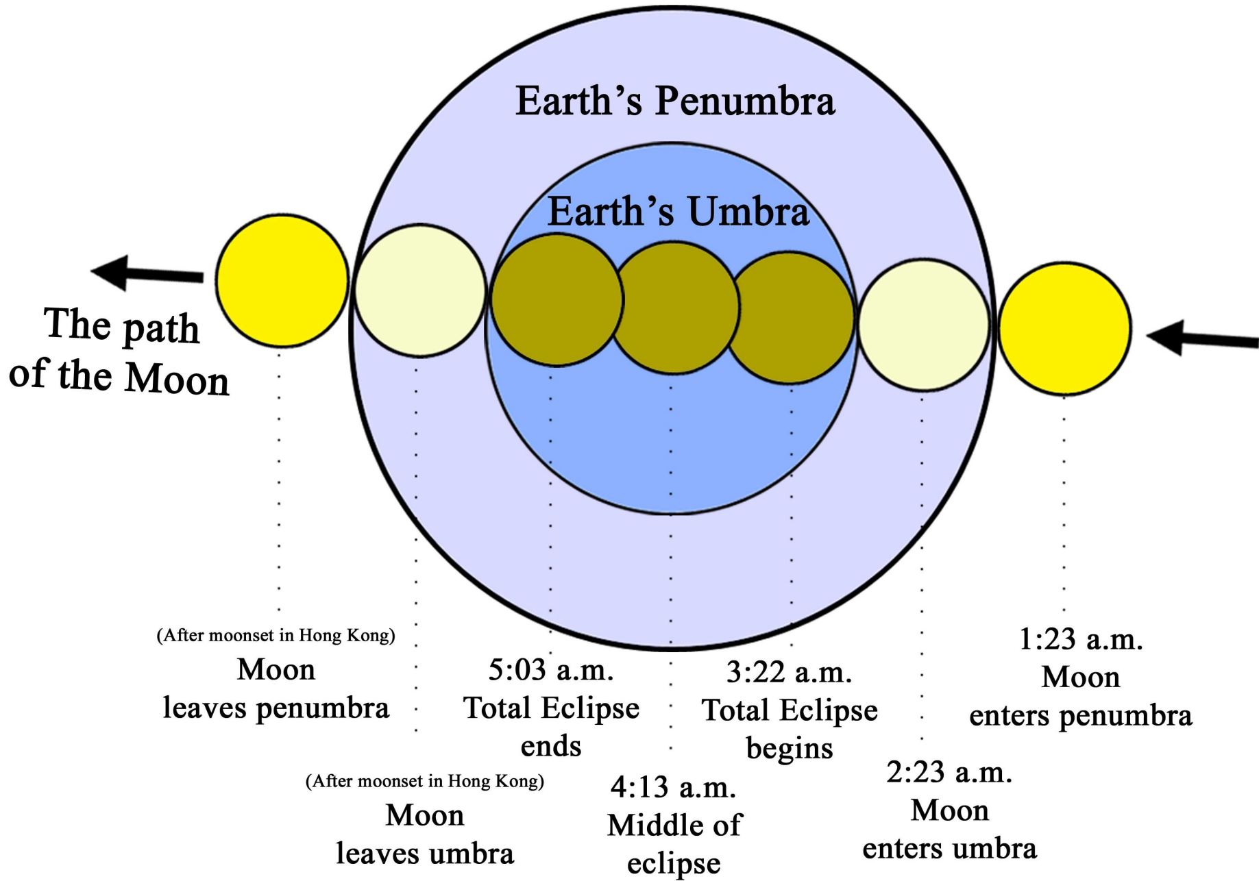
The path of the moon during the eclipse on 16 June 2011
