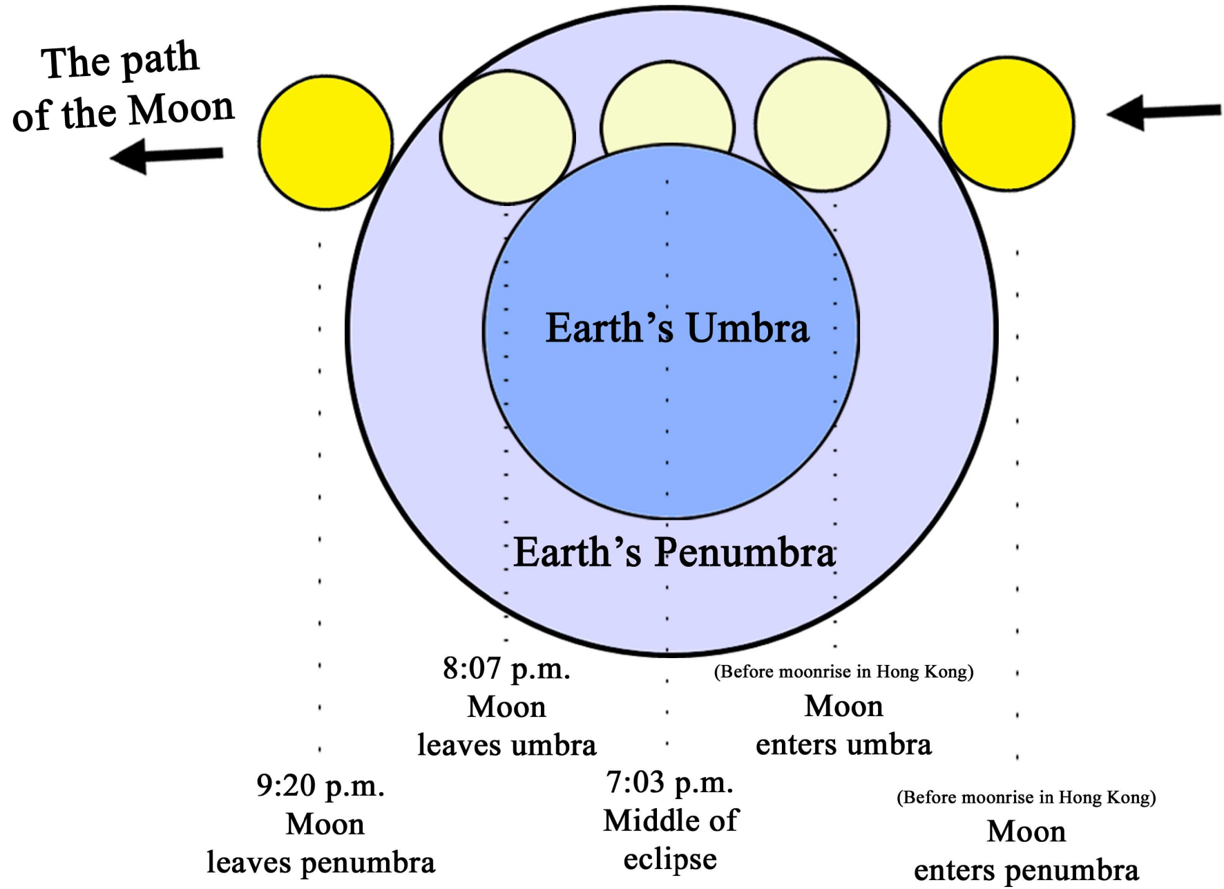
The path of the moon during the eclipse on June 4, 2012
