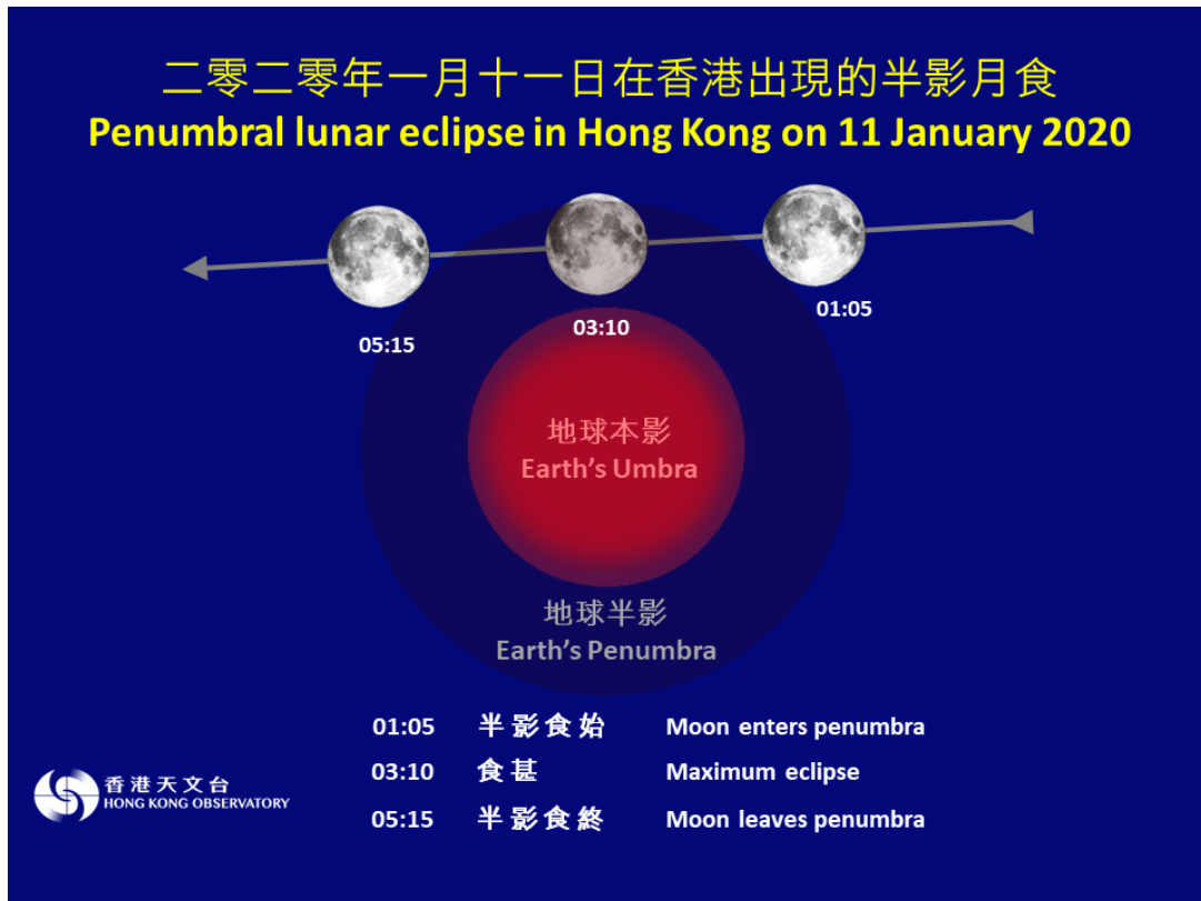
Figure 1 The penumbral lunar eclipse process on January 11, 2020
