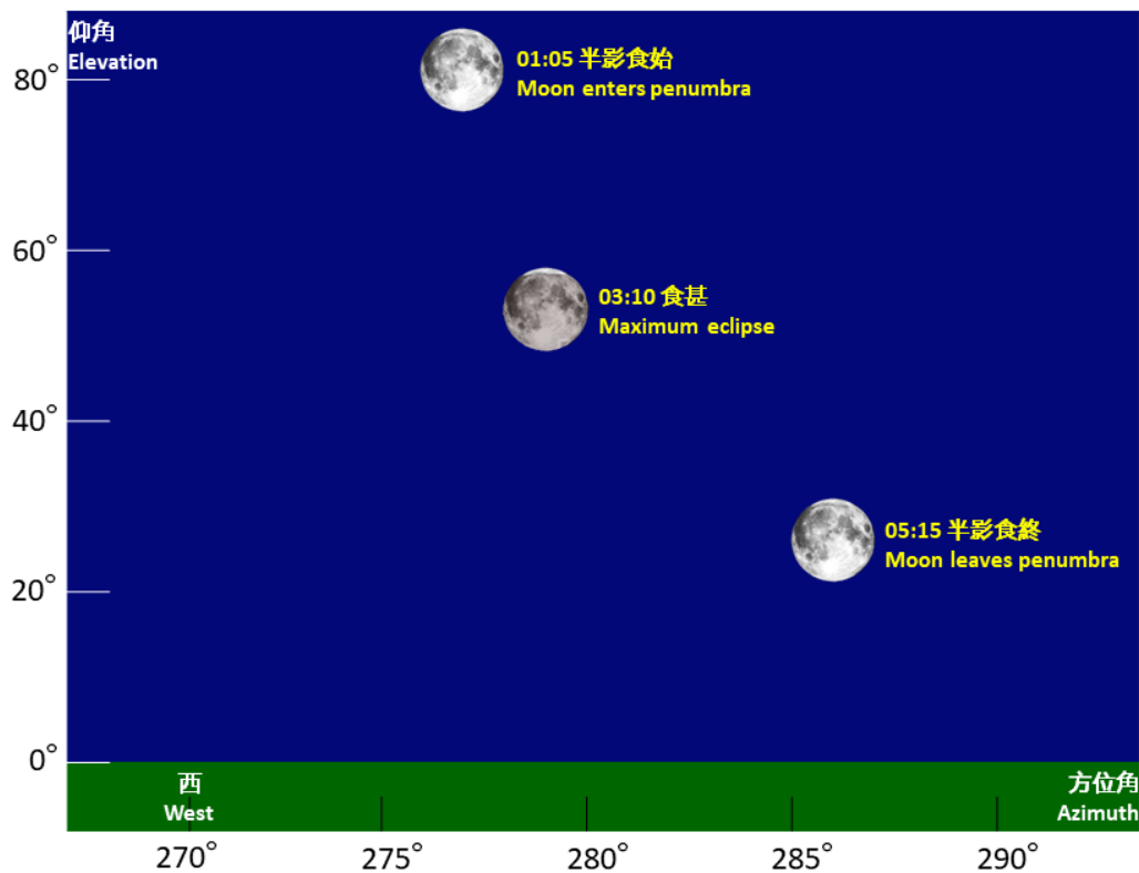
Figure 2 Schematic diagram showing elevation and azimuth of the moon during the penumbral eclipse on January 11, 2020
