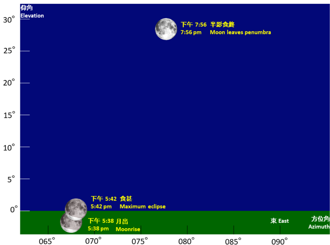
Figure 2 Schematic diagram showing elevation and azimuth of the Moon during the penumbral eclipse on November 30, 2020
