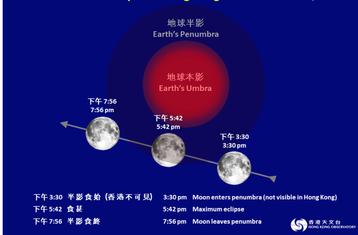
Figure 1 The penumbral lunar eclipse process on November 30, 2020
