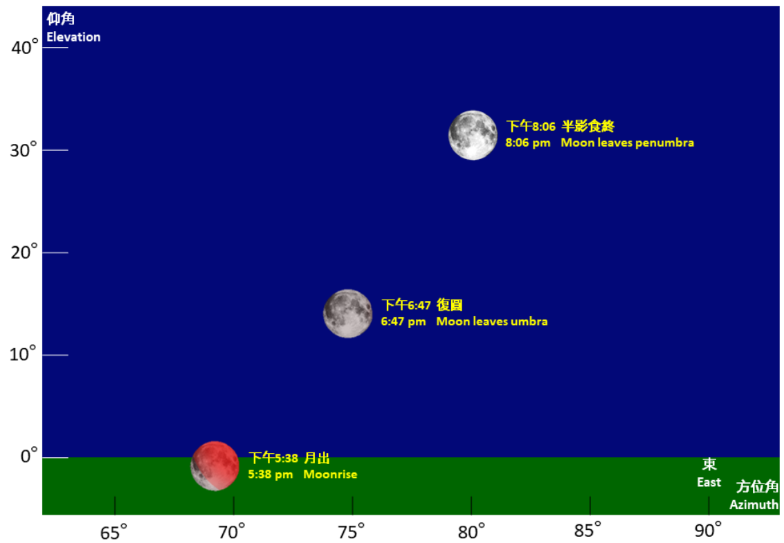
Figure 2 Schematic diagram showing elevation and azimuth of the moon during the partial eclipse on November 19, 2021
