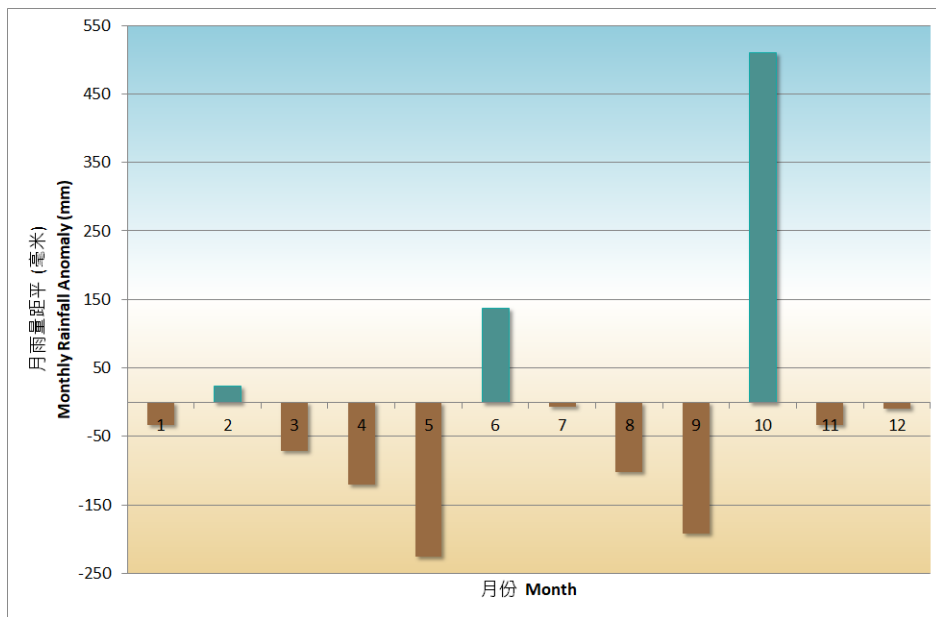
Figure 6 Monthly rainfall anomalies (against the 1991-2020 normal) in Hong Kong in 2021
