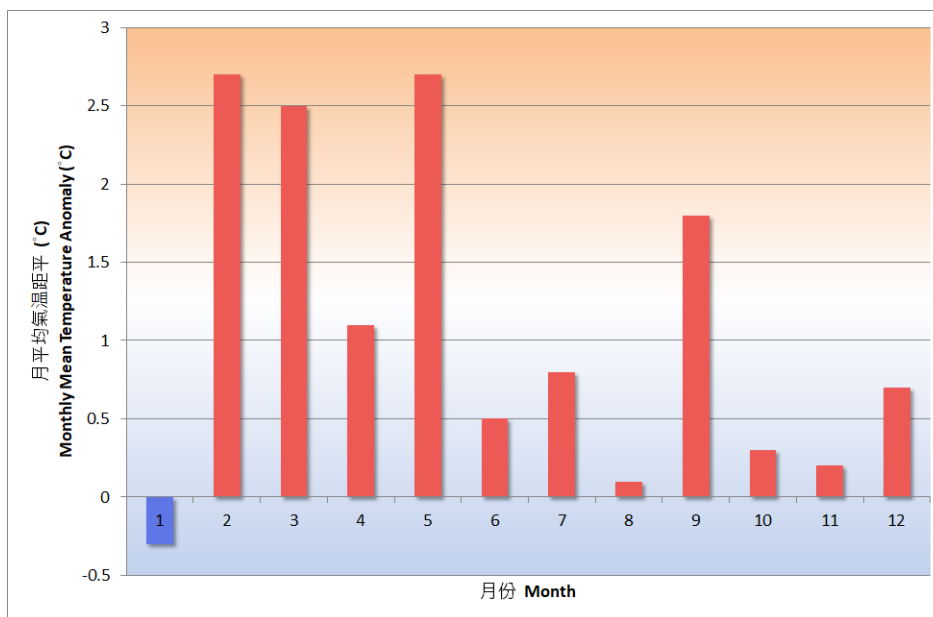
Figure 1 Monthly mean temperature anomalies (against the 1991-2020 normal) in Hong Kong in 2021
