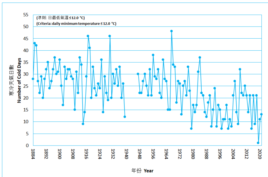
Figure 4 Long-term time series of number of Cold Days in Hong Kong (1884-2021)
