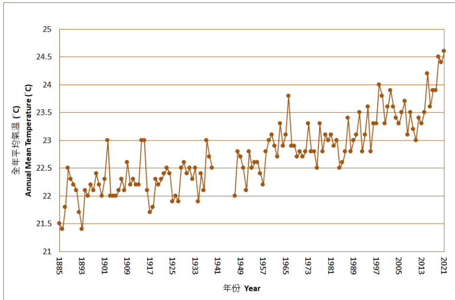
Figure 5 Long-term time series of annual mean temperature in Hong Kong (1885-2021)
