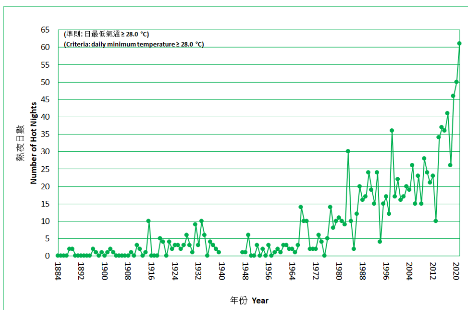
Figure 2 Long-term time series of number of Hot Nights in Hong Kong (1884-2021)
