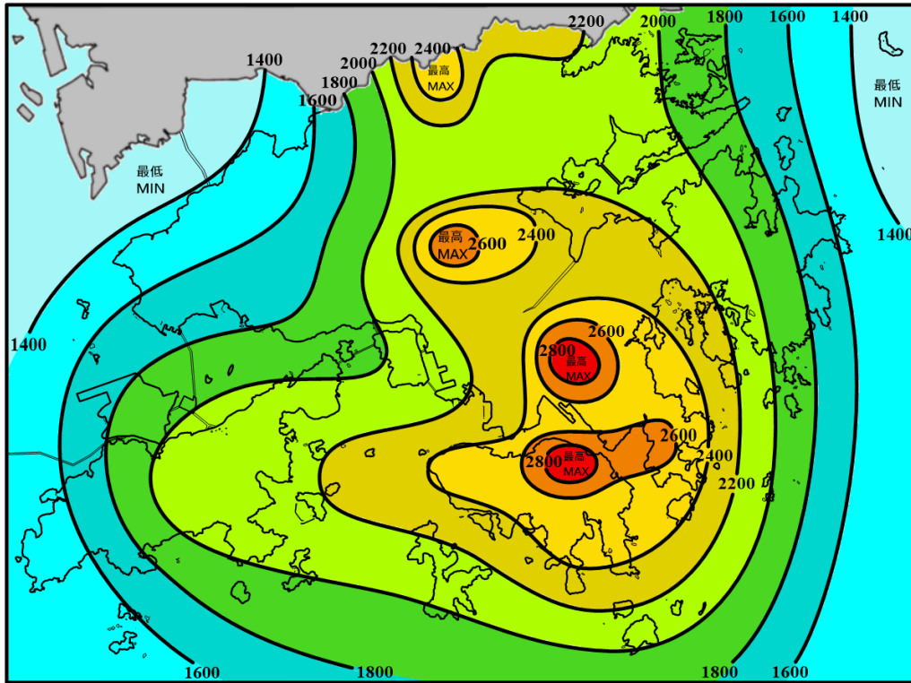
Figure 7 Annual rainfall distribution (millimetres) in Hong Kong in 2021
