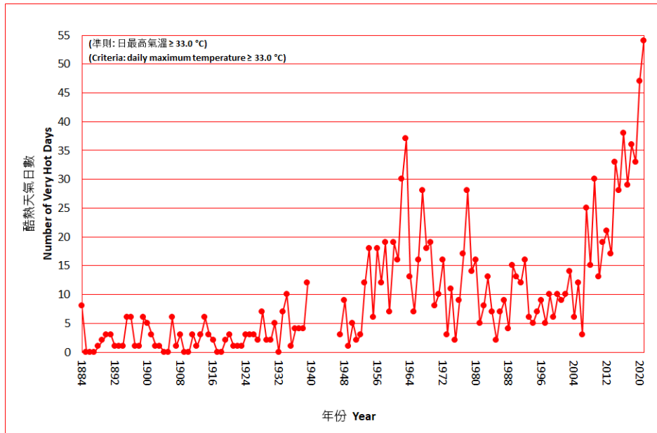
Figure 3 Long-term time series of number of Very Hot Days in Hong Kong (1884-2021)
