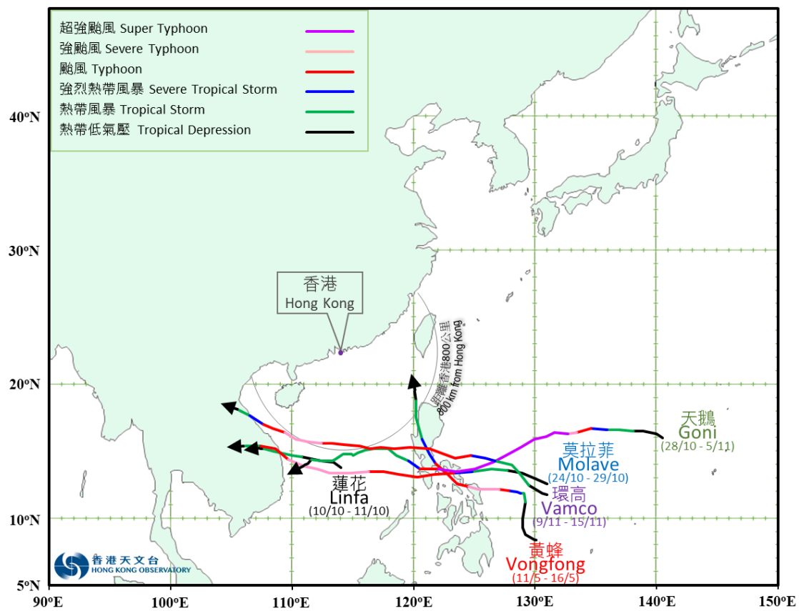
Tracks of Vongfong, Linfa, Molave, Goni and Vamco in 2020
