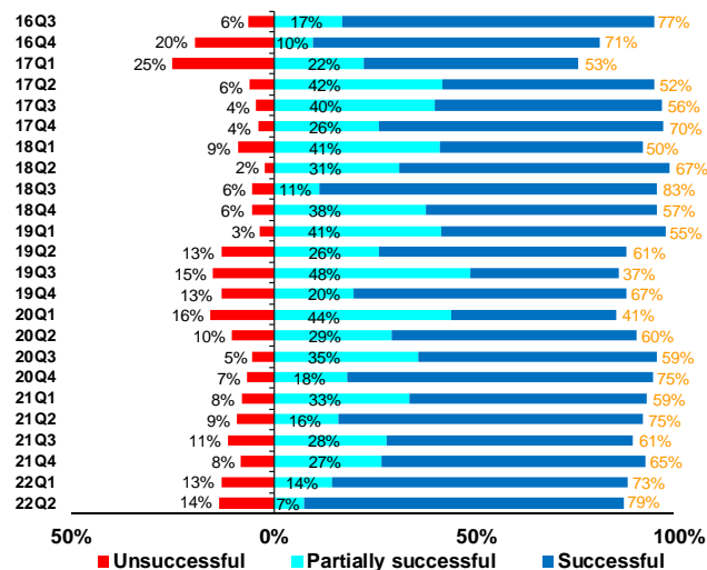
Chart 3: Results of new bank credit applications
