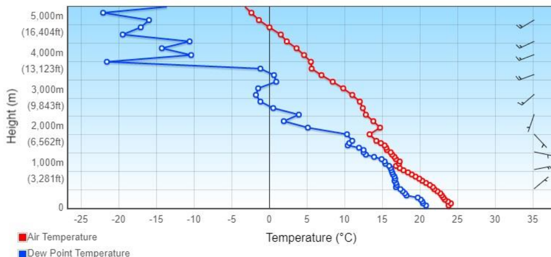
Figure 2 As shown in the upper-air weather data at the night of 17 November 2022, the air and dew point temperatures at around 1000 m height were very close to each other, suggesting the possible presence of clouds. This height generally matched the cloud base height over Pat Sin Leng observed at around 5 p.m. in Figure 1.
