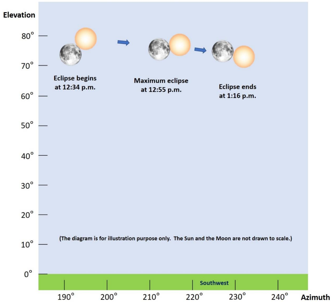
Schematic diagram showing the elevation and azimuth of the sun and the moon during the partial solar eclipse on April 20, 2023
