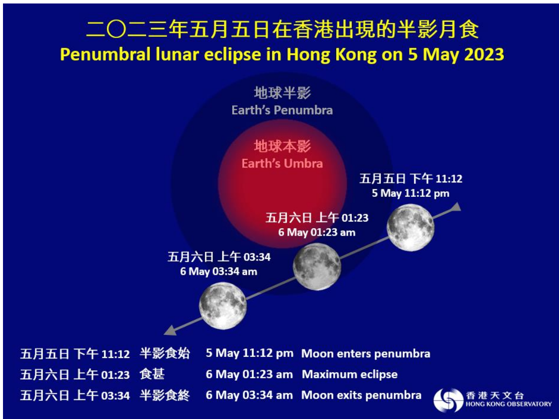
Figure 1. The penumbral lunar eclipse process on May 5, 2023.
