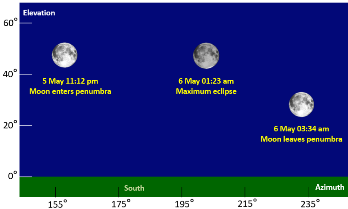
Figure 2. A schematic diagram showing the elevation and azimuth of the moon during the penumbral eclipse on May 5, 2023.
