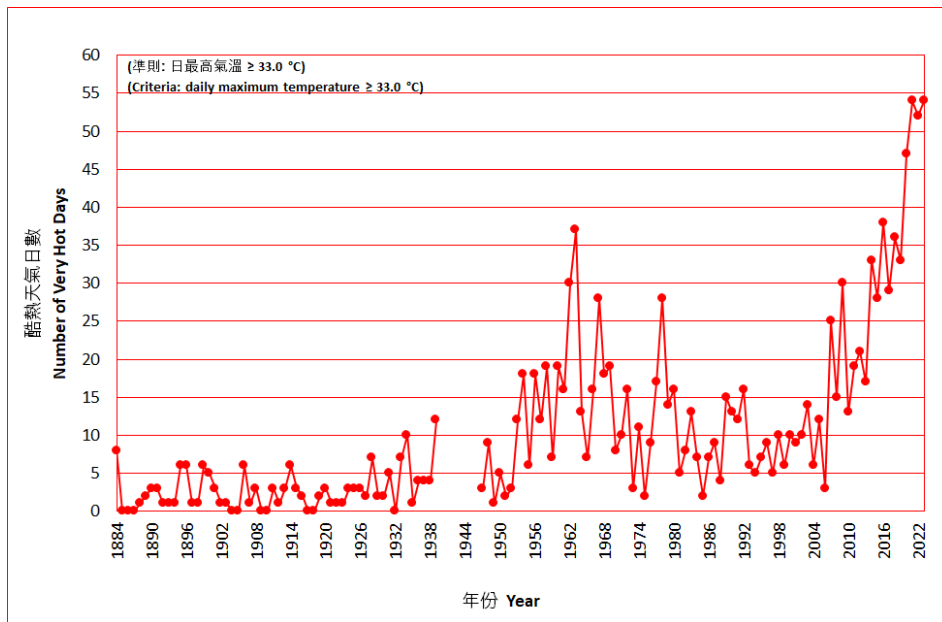
Figure 3 Long-term time series of number of very hot days in Hong Kong 1884-2023
