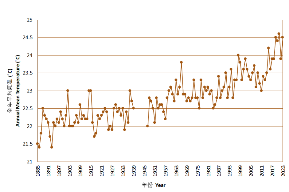
Figure 6 Long-term time series of annual mean temperature in Hong Kong 1885-2023
