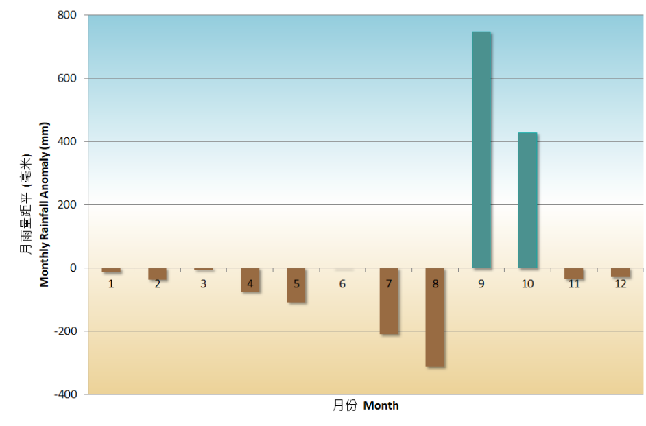
Figure 7 Monthly rainfall anomalies (against the 1991-2020 normal) in Hong Kong in 2023
