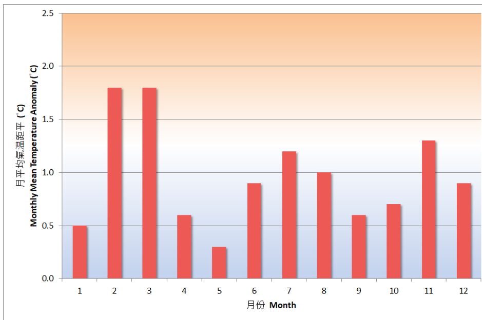
Figure 1 Monthly mean temperature anomalies (against the 1991-2020 normal) in Hong Kong in 2023
