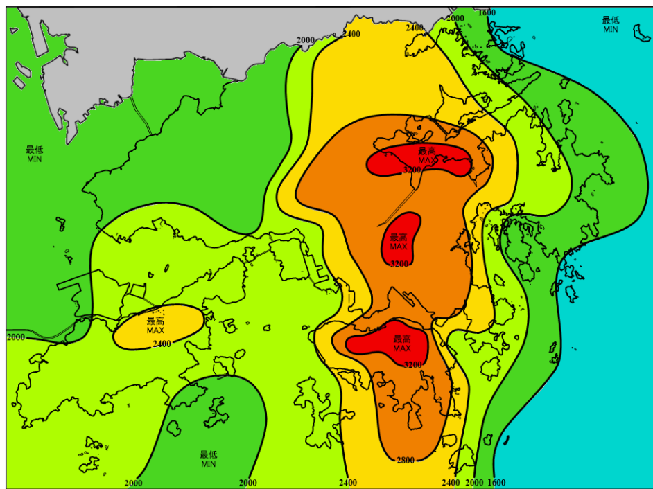
Figure 8 Annual rainfall distribution in Hong Kong in 2023 (in millimetres)
