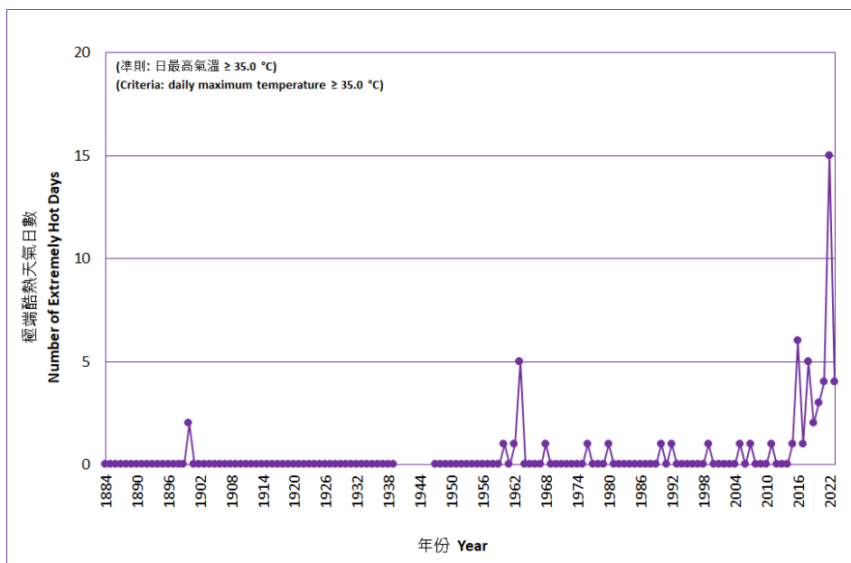
Figure 4 Long-term time series of number of extremely hot days in Hong Kong 1884-2023
