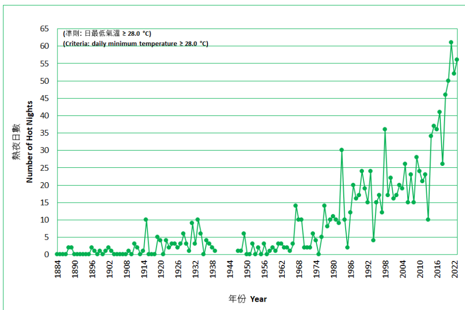
Figure 2 Long-term time series of number of hot nights in Hong Kong 1884-2023
