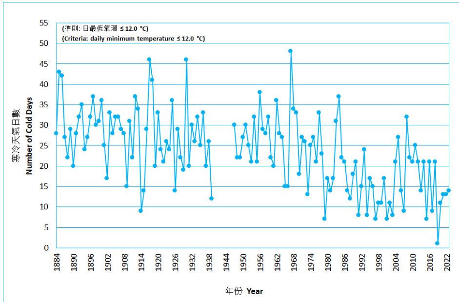
Figure 5 Long-term time series of number of cold days in Hong Kong 1884-2023
