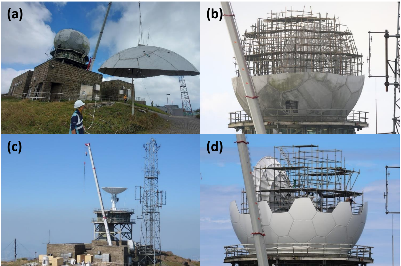
Figure 3 (a) Dismantling the radome of the old Tai Mo Shan weather radar (TMSWR), (b) building a scaffolding for removing the antenna of the old TMSWR, (c) installing antenna and pedestal for the new TMSWR and (d) the new radome under construction.
