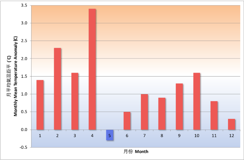
Figure. 1 Monthly mean temperature anomalies (against the 1991-2020 normal) in Hong Kong in 2024
