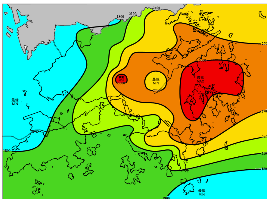
Figure 8 Annual rainfall distribution in Hong Kong in 2024 (in millimetres)
