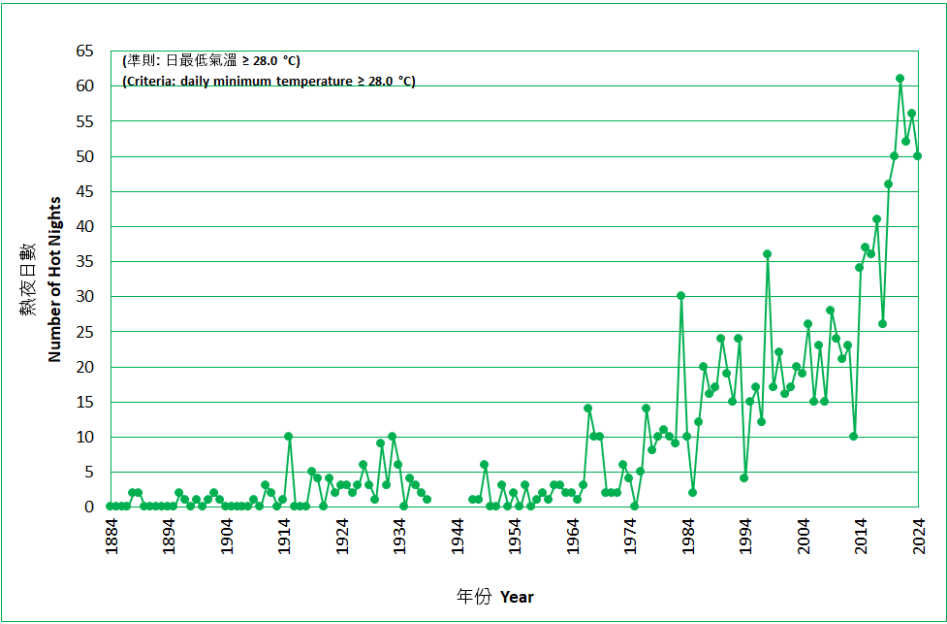
Figure 2 Long-term time series of number of hot nights in Hong Kong (1884-2024)
