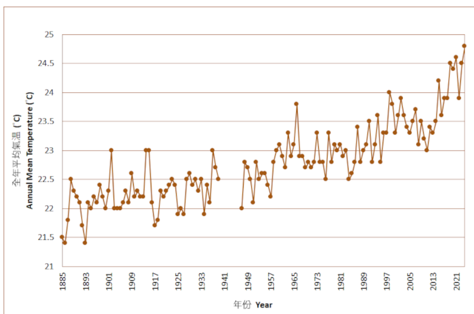
Figure 6 Long-term time series of annual mean temperature in Hong Kong (1885-2024)
