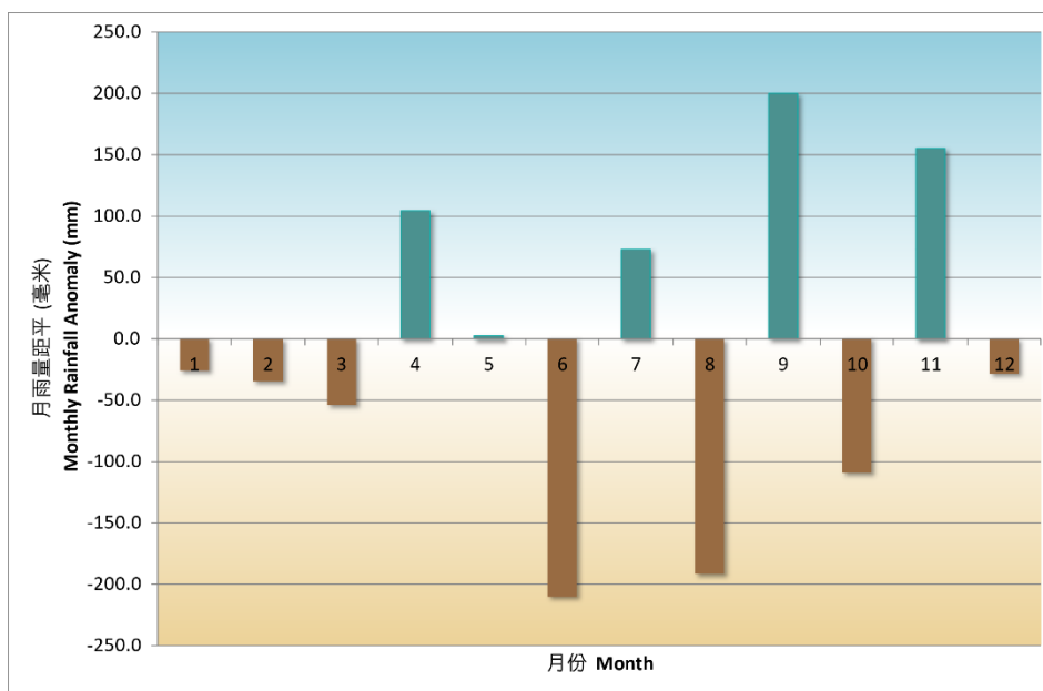
Figure 7 Monthly rainfall anomalies (against the 1991-2020 normal) in Hong Kong in 2024
