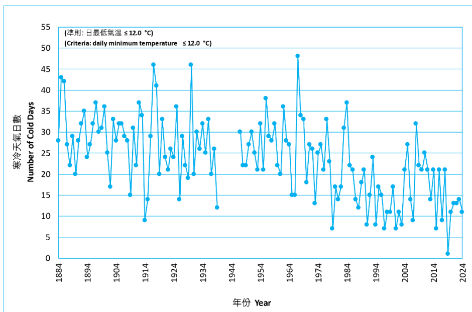
Figure 5 Long-term time series of number of cold days in Hong Kong (1884-2024)
