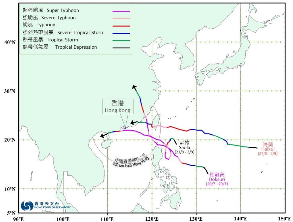
Tracks of tropical cyclones Doksuri, Saola and Haikui in 2023
