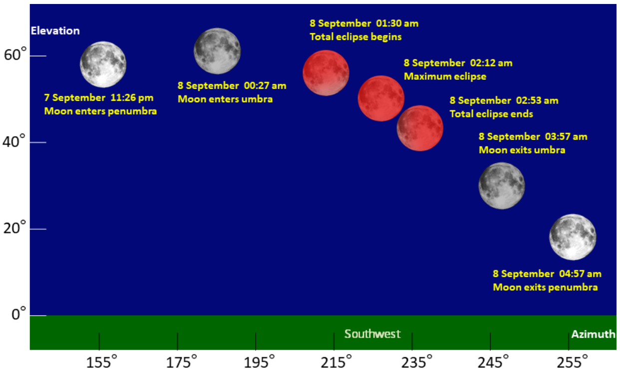
Figure 2 Schematic diagram showing elevation and azimuth of the moon during the eclipse on September 7 to 8, 2025.
