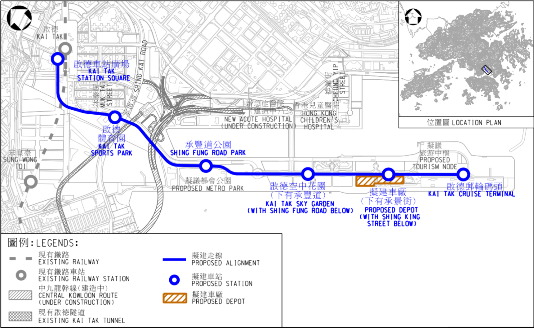
Proposed Alignment of Smart and Green Mass Transit System in Kai Tak
