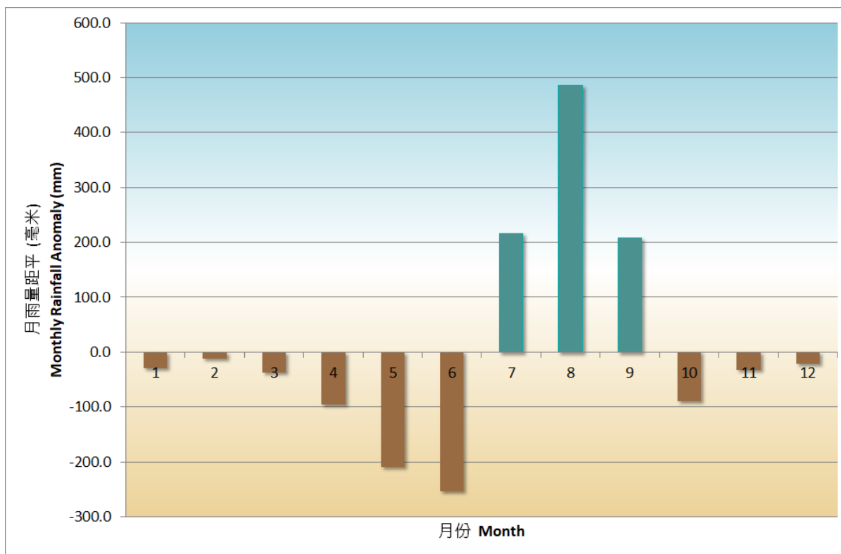
Figure. 7 Monthly rainfall anomalies (against the 1991-2020 normal) in Hong Kong in 2025
