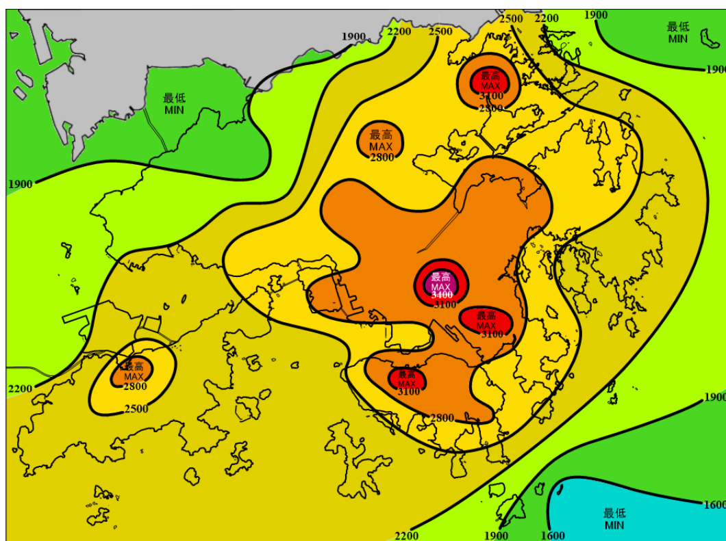
Figure. 8 Annual rainfall distribution in Hong Kong in 2025 (in millimetres)
