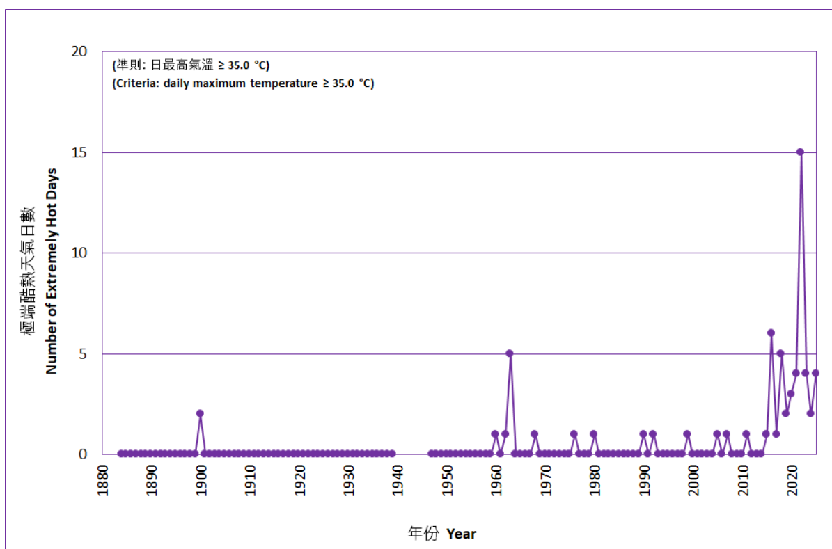
Figure. 4 Long-term time series of number of extremely hot days in Hong Kong (1884-2025)
