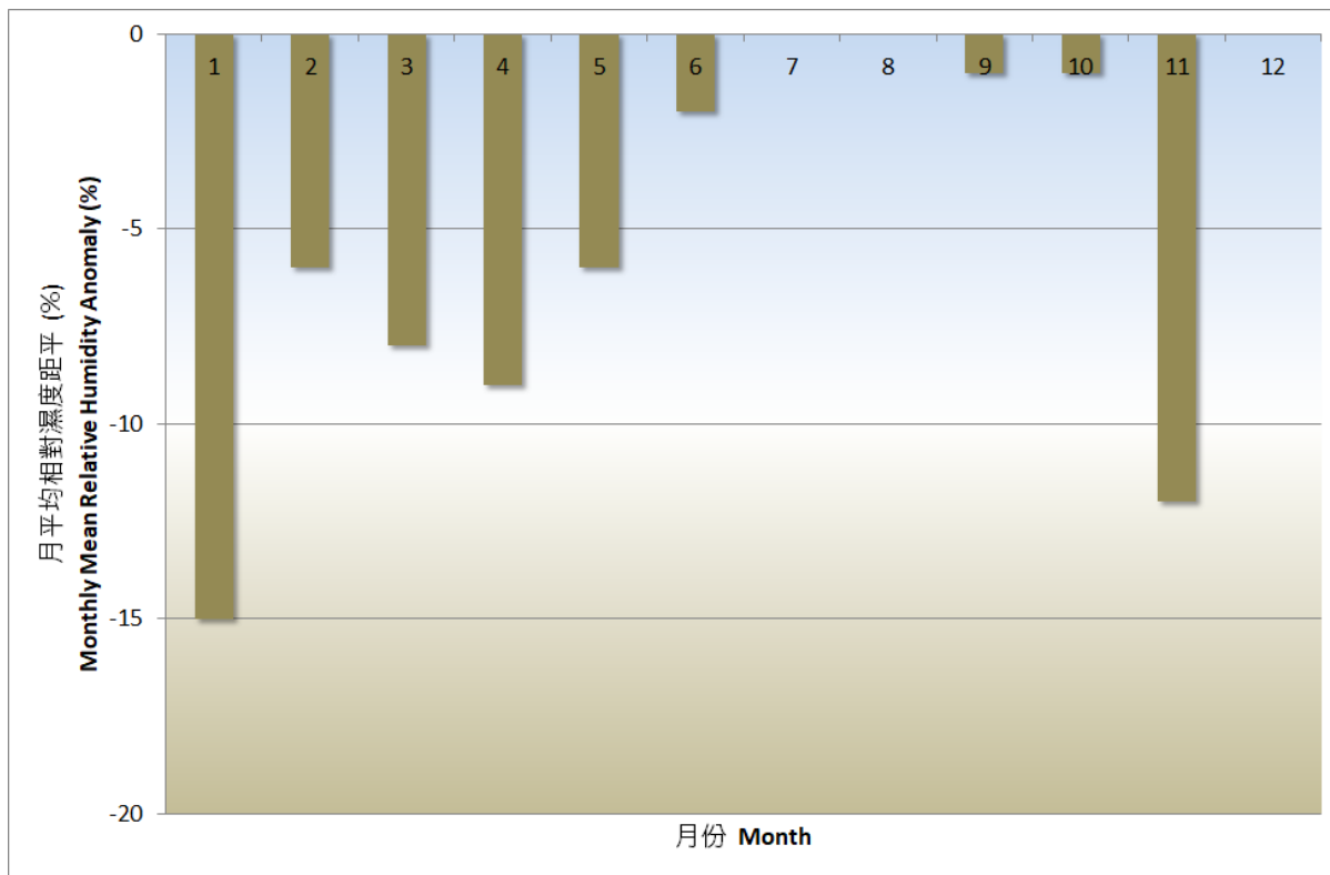
Figure. 9 Monthly mean relative humidity anomalies (against the 1991-2020 normal) in Hong Kong in 2025
