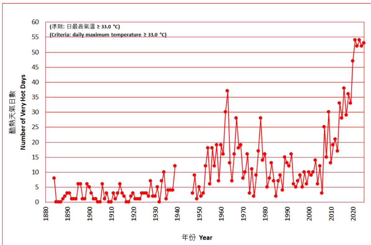
Figure. 3 Long-term time series of number of very hot days in Hong Kong (1884-2025)
