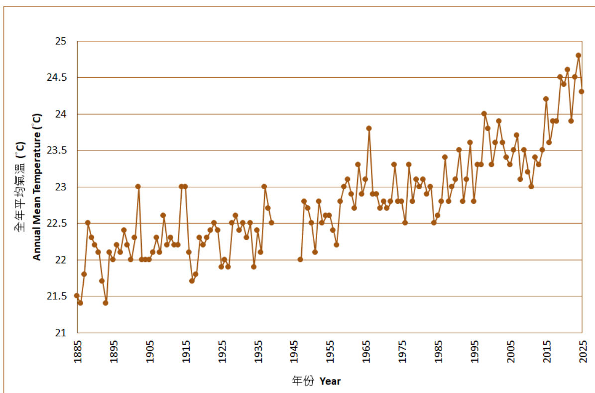
Figure. 6 Long-term time series of annual mean temperature in Hong Kong (1885-2025)
