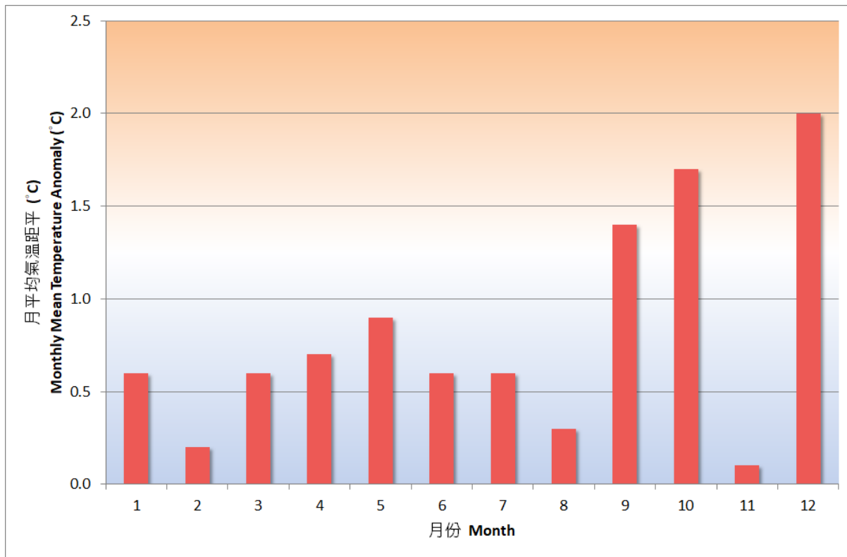
Figure. 1 Monthly mean temperature anomalies (against the 1991-2020 normal) in Hong Kong in 2025
