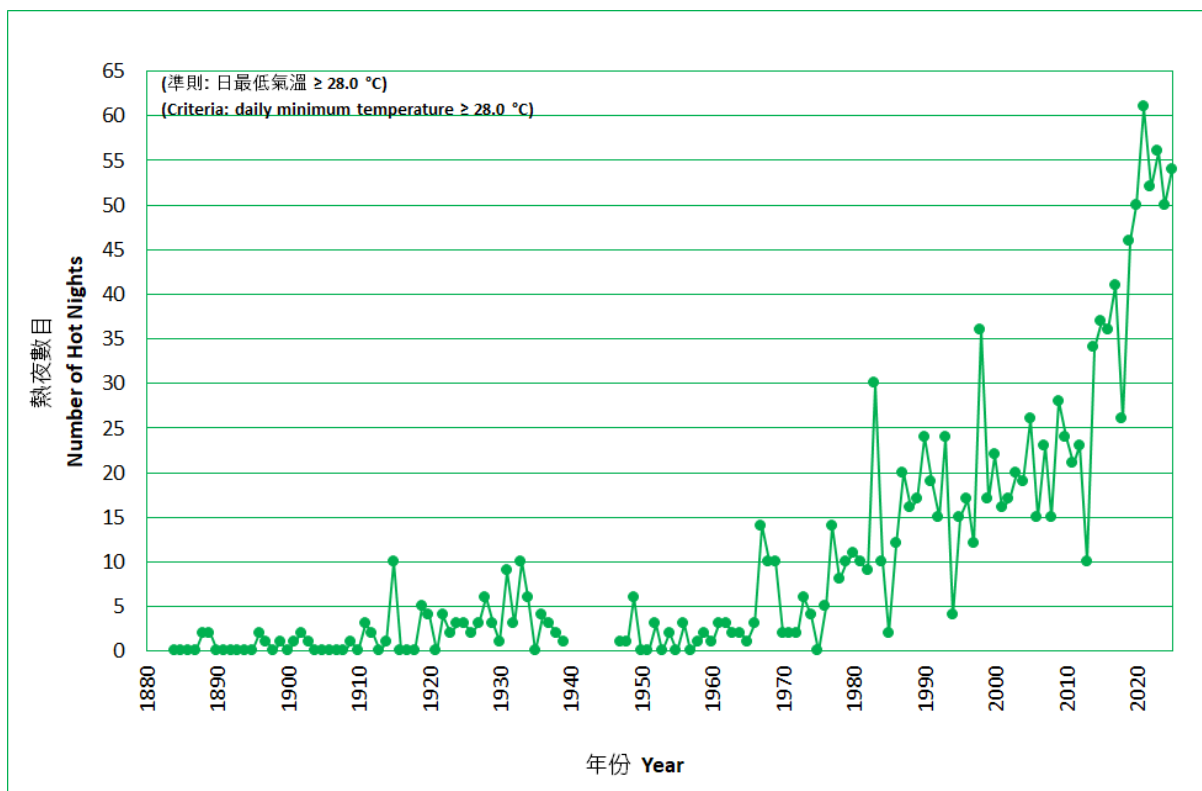
Figure. 2 Long-term time series of number of hot nights in Hong Kong (1884-2025)
