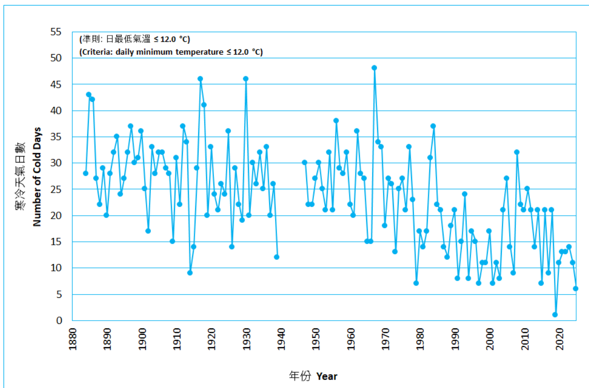
Figure. 5 Long-term time series of number of cold days in Hong Kong (1884-2025)
