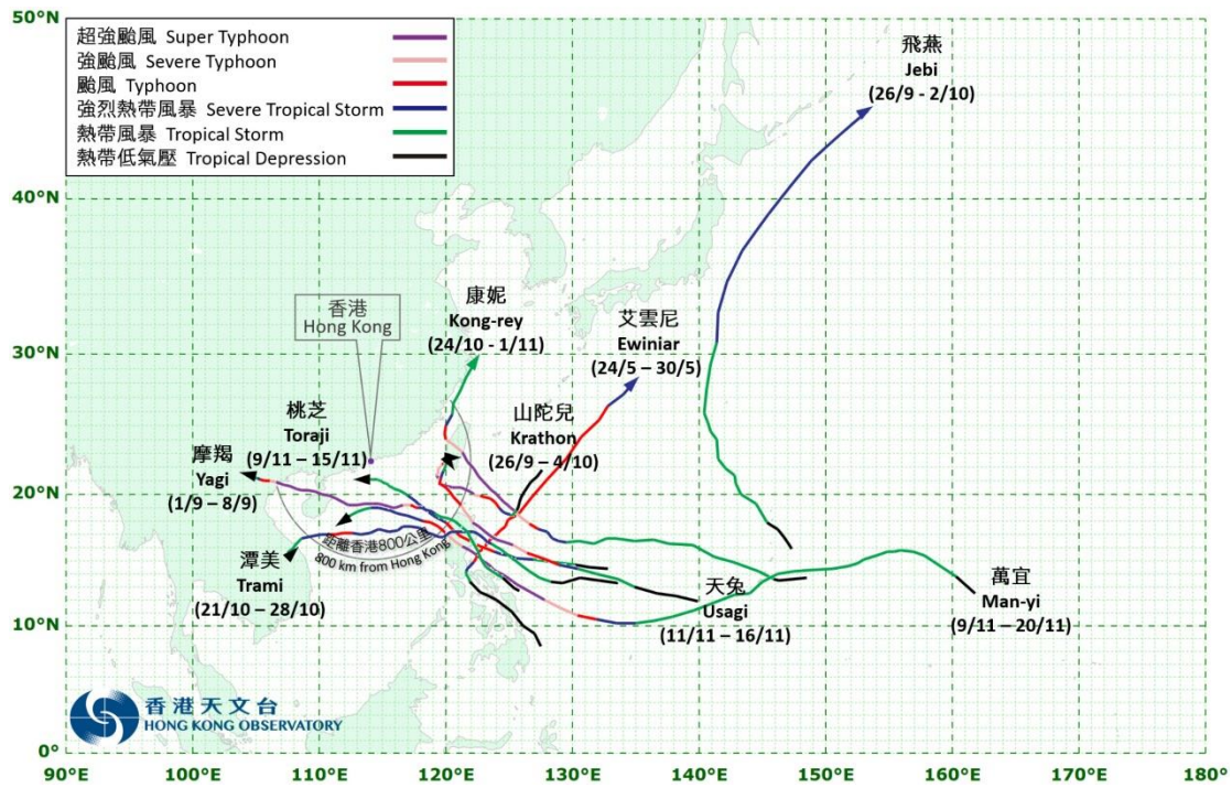
Tracks of tropical cyclones Kong-rey, Toraji, Man-yi, Usagi, Yagi, Ewiniar, Jebi, Krathon and Trami in 2024
